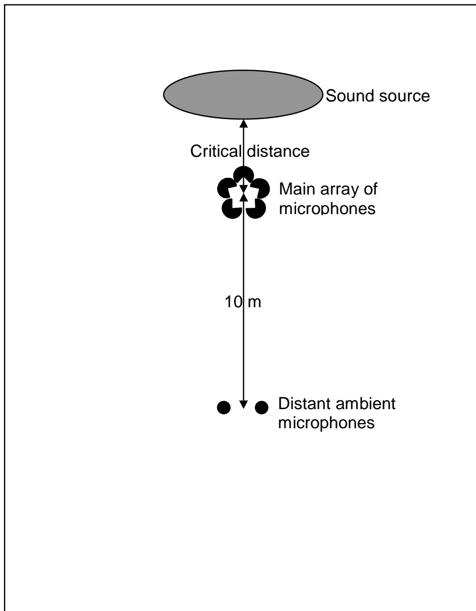
Figure 1: Diagram of microphone layout.
